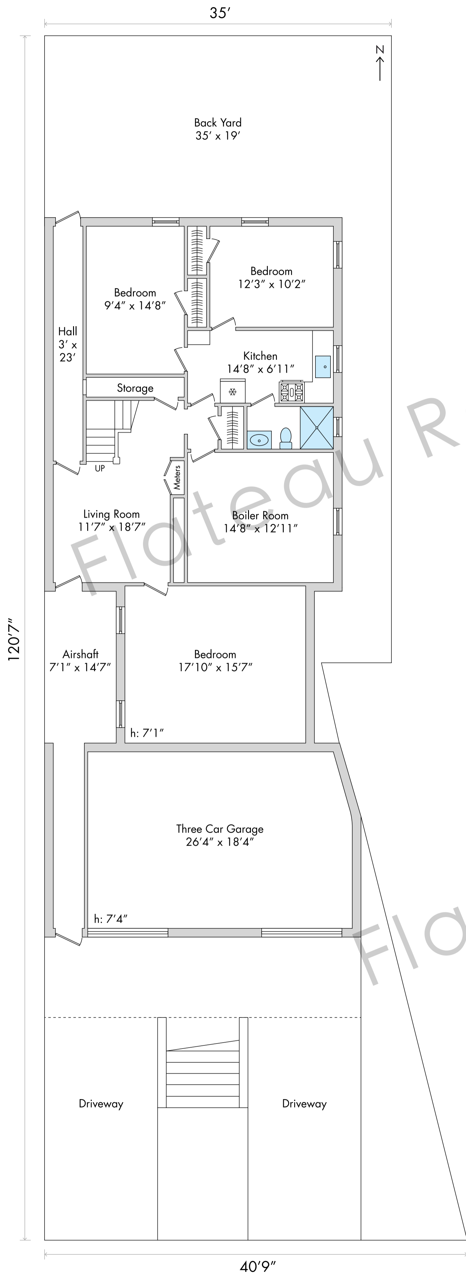
FIRST FLOOR
