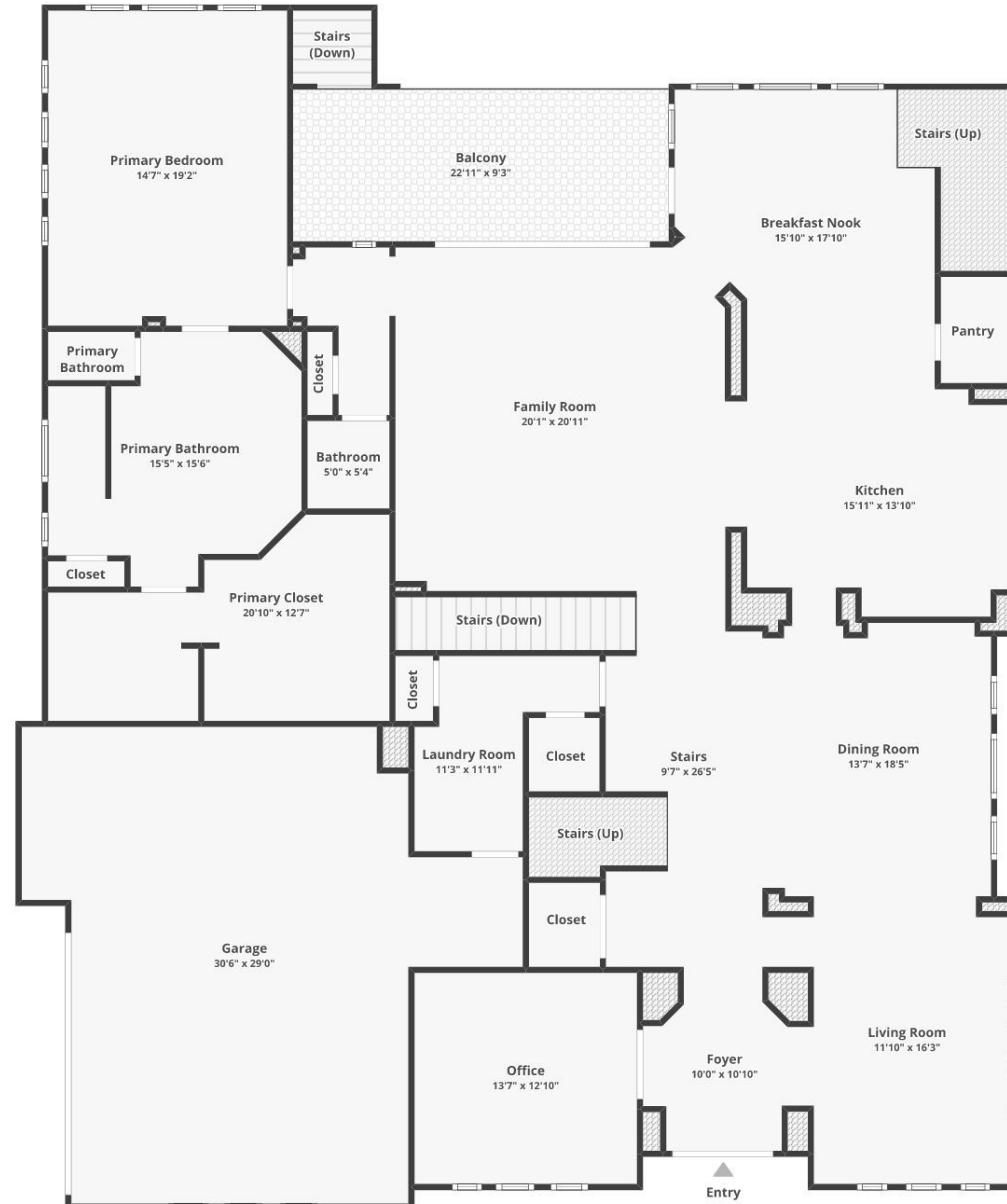
FLOOR 2
