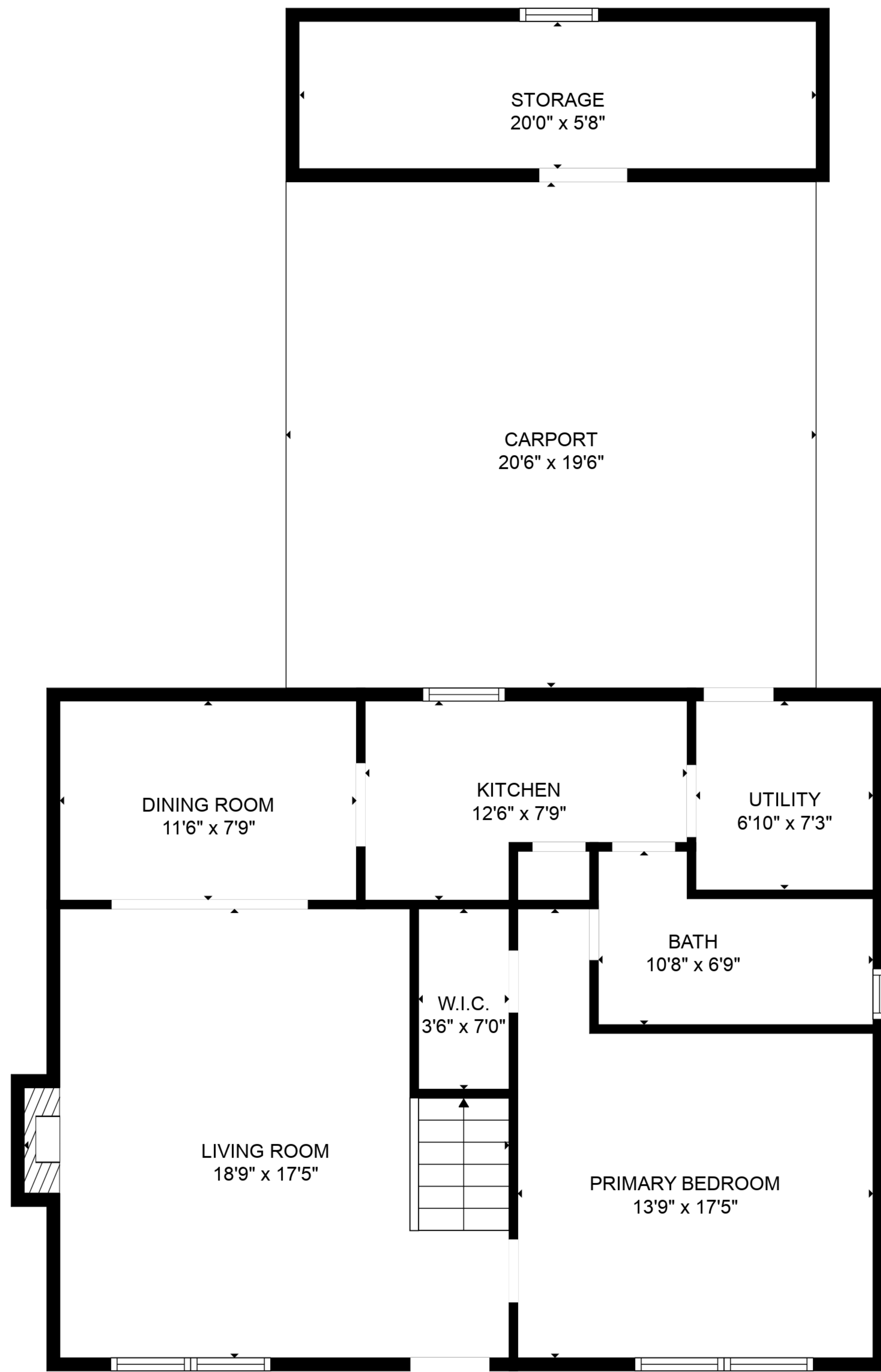
FLOOR 1
