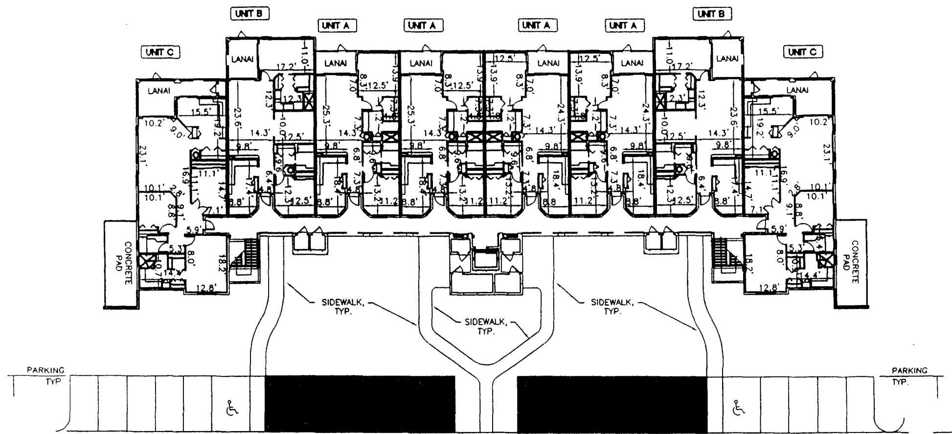
FIRST FLOOR BUILDING PLAN
