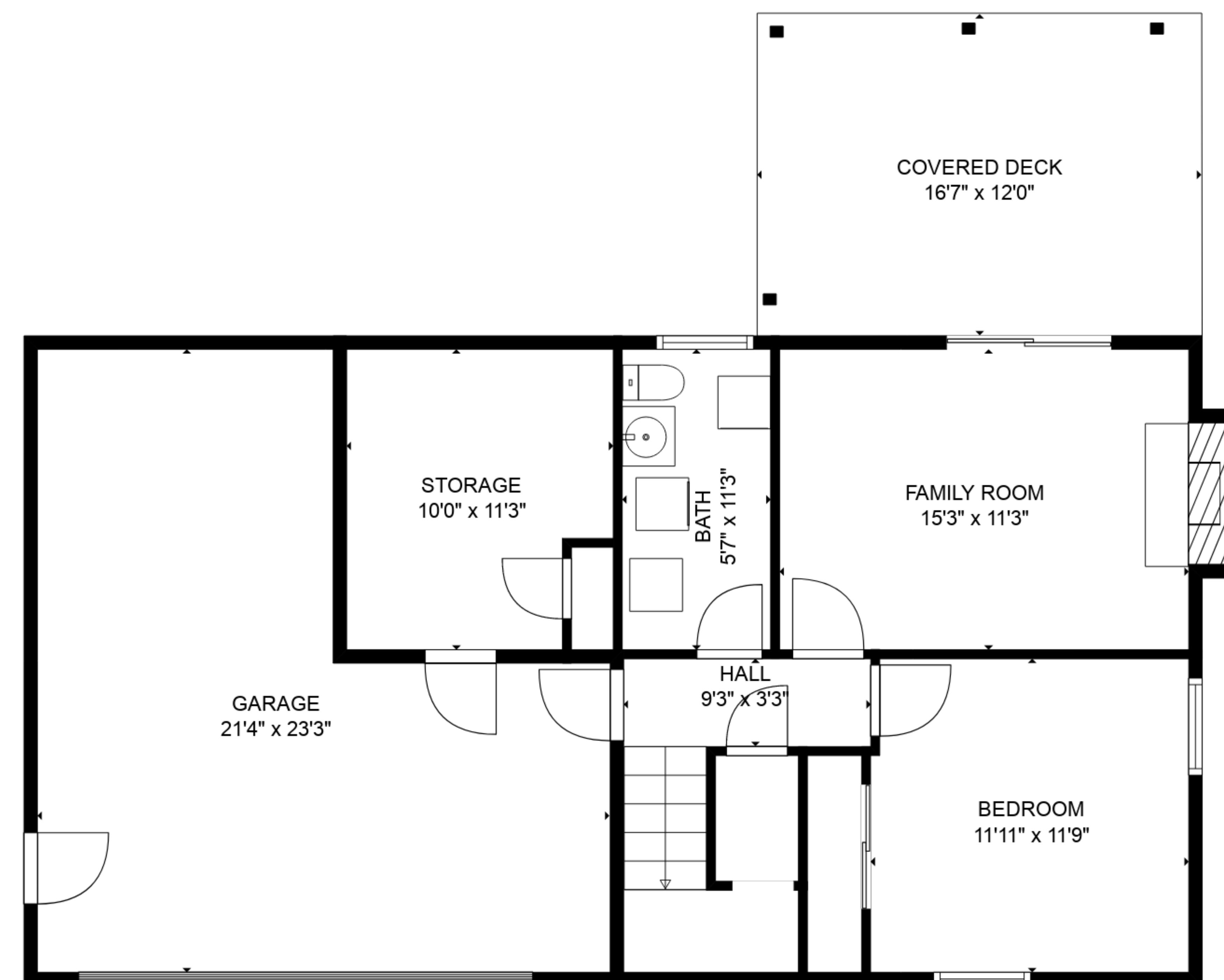
FLOOR 2
