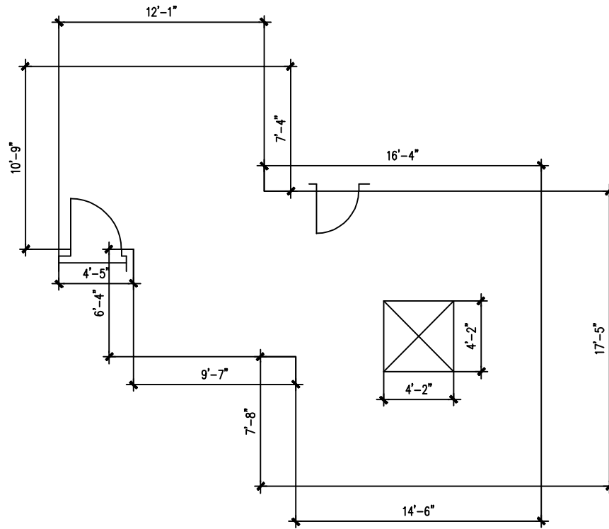
HOBBY ROOM FLOOR AREA 430 SQ FT +/-
