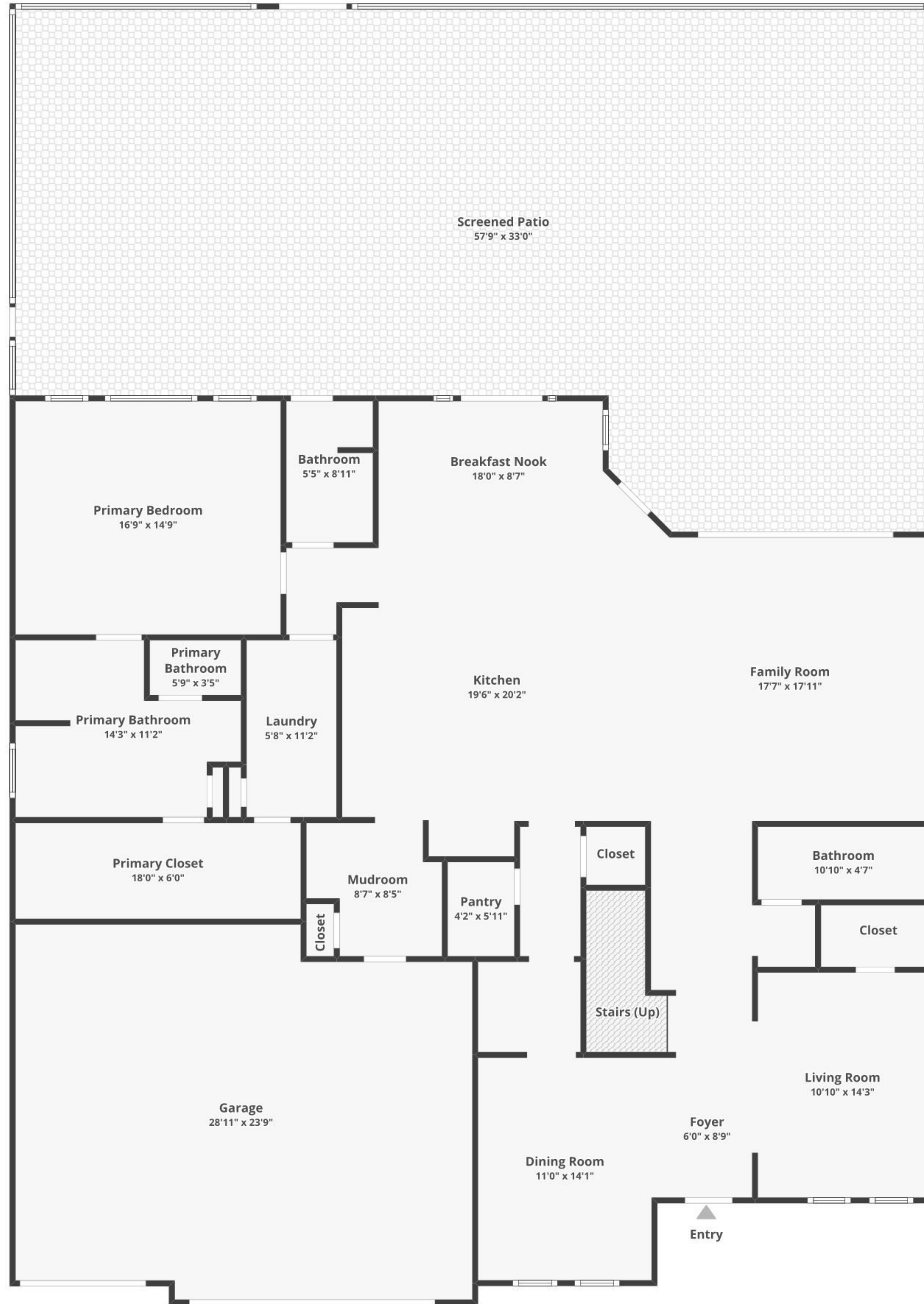
FLOOR 1
