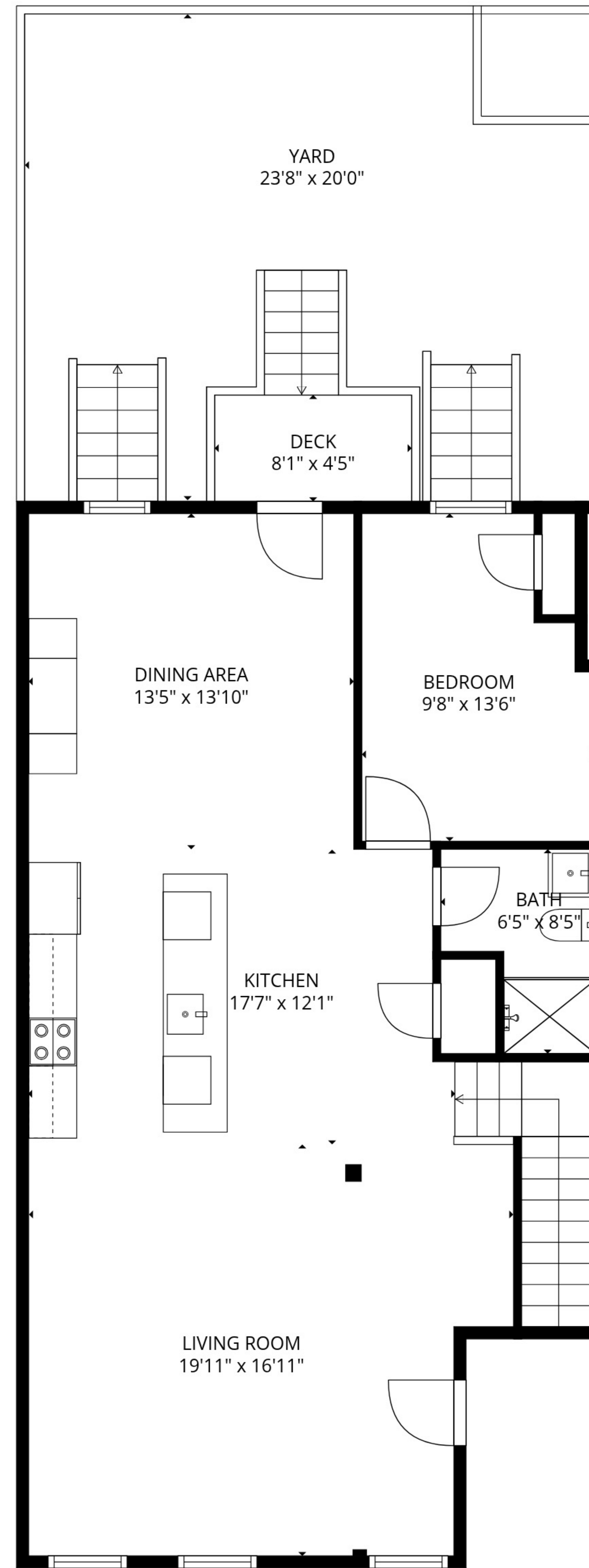
2nd floor
