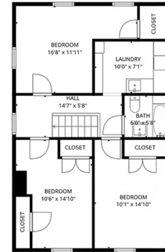
4th floor
